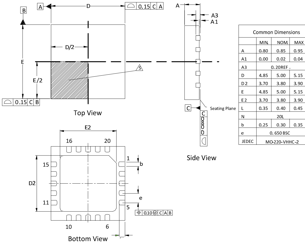
Figure 34 - Physical Dimensions
